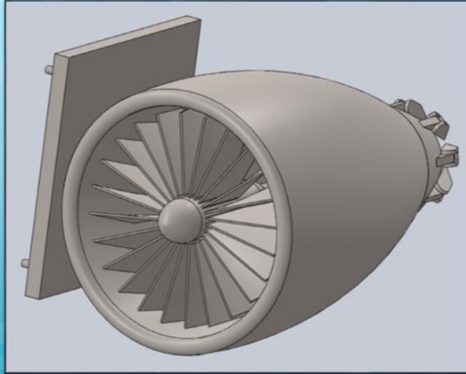
Turbine Sub-Assembly
